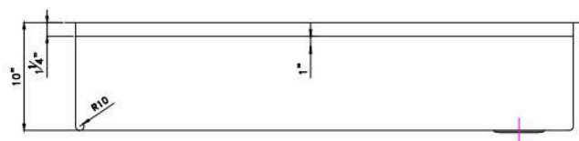
Side section view
